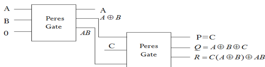
Figure2: Block Diagram of 1-bit Full Adder
