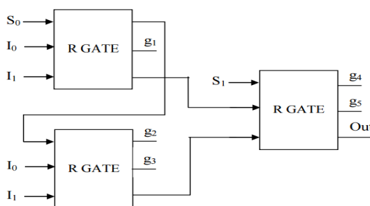
Figure 5: Proposed Diagram of 4×1 Multiplexer
