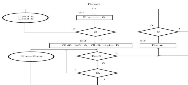
Figure 4: ASM Flow Chart of Multiplier
