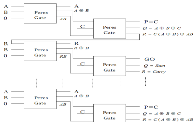
Figure 3: Block Diagram of n-bit Full Adder
